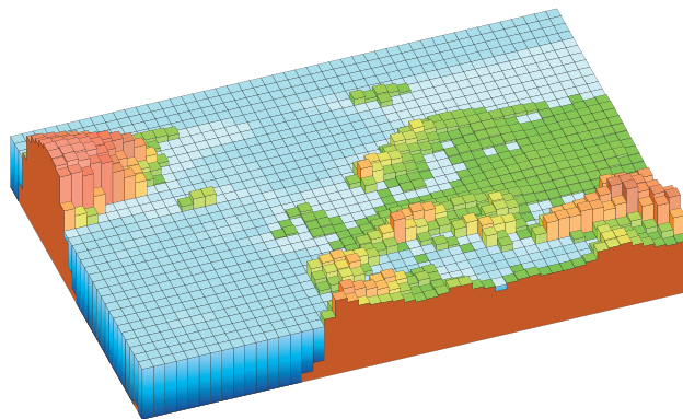
Grid spacing approximately 180 km
