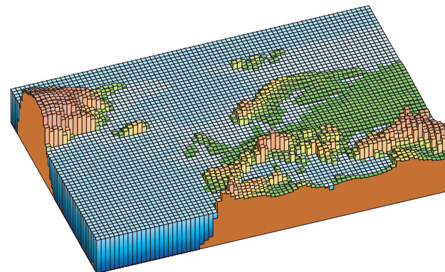
Grid spacing approximately 110 km
